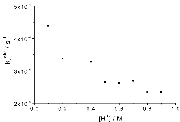
Figure 6. k_1^{\text{obs}} [ \text{s}^{-1} ] as a function of [\text{H}^+] [M] in the acid hydrolysis kinetics of \text{FeL}^4 ; [\text{FeL}^4] = 0.1 \text{ mM} ; solvent: water, I = 2 \text{ M} ( \text{NaClO}_4 , \text{HClO}_4 ), 25^\circ\text{C}
