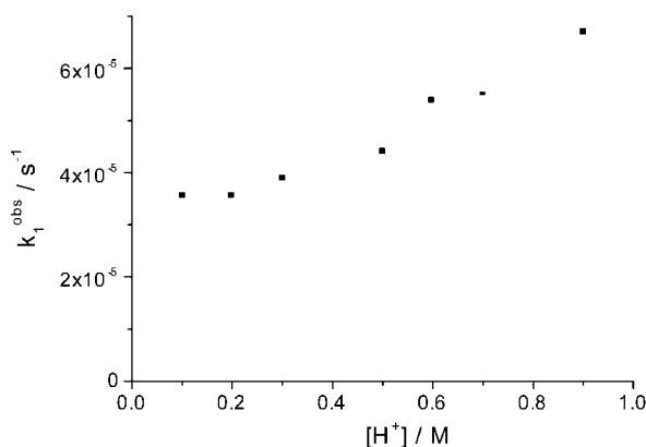
Figure 7. k_1^{\text{obs}} [s -1 ] as a function of [H + ] [M] in the acid hydrolysis kinetics of FeL 0 ; [FeL 0 ] = 0.07 mM; solvent: water, I = 2 M (NaClO 4 , HClO 4 ), 25 °C
