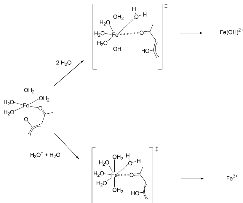
Figure 12. Transition states for proton-dependent and proton-independent dissociation of bidentate \text{Fe}-\text{L}^n complexes
