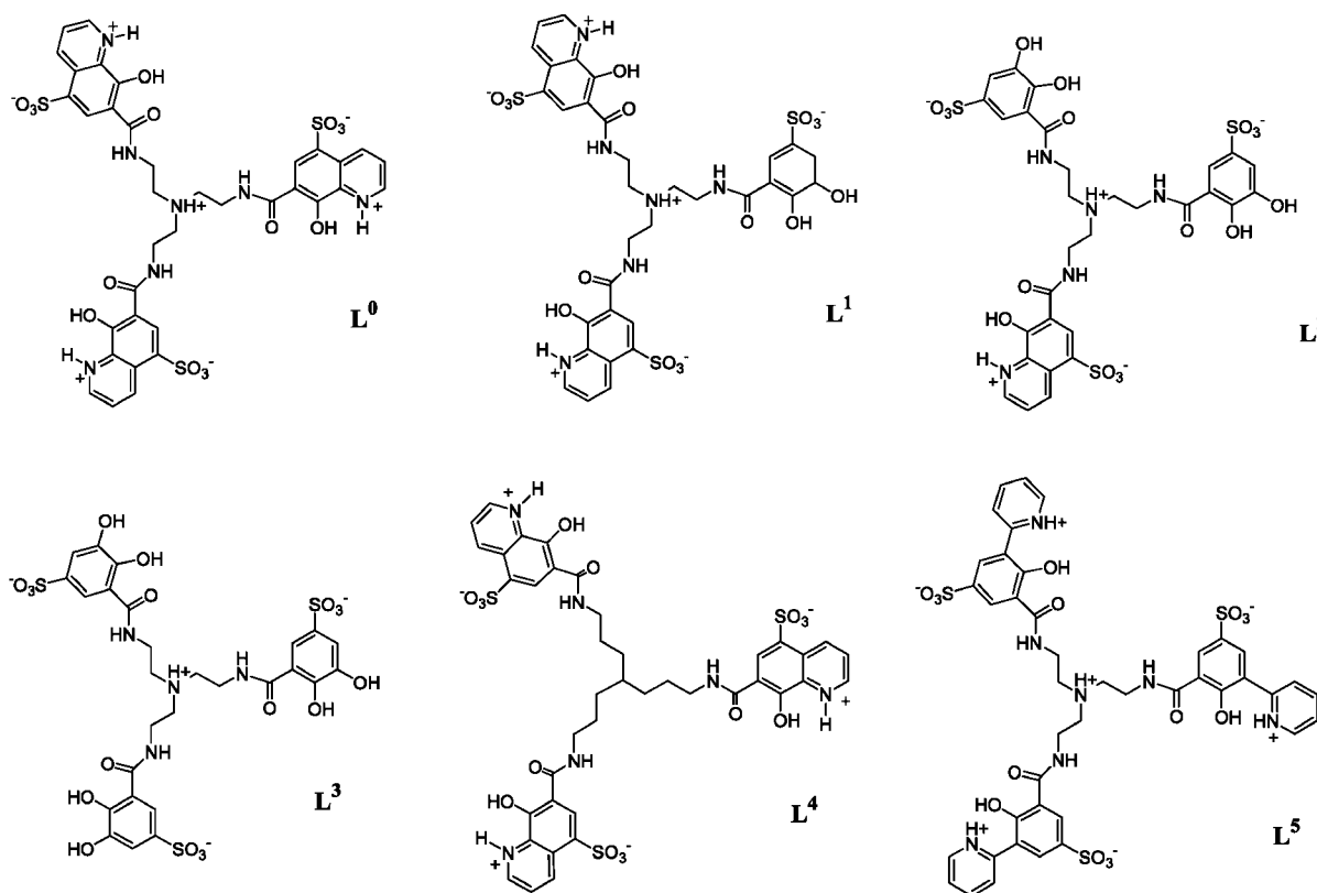
Figure 1. Chemical formulae of the tripodal ligands
