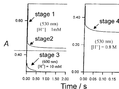
Figure 3. Acid hydrolysis kinetics of the \text{Fe}^{\text{III}}\text{L}^2 complex: absorbance decay at \lambda = 530 or 600 nm; [\text{Fe}^{\text{III}}\text{L}^2] = 0.05 mM; [\text{H}^+] = 1 mM for stages 1 and 2, [\text{H}^+] = 10 mM for stage 3, [\text{H}^+] = 0.8 M for stage 4; solvent: water, I = 2 M ( \text{NaClO}_4 , \text{HClO}_4 ), 25^\circ\text{C}
