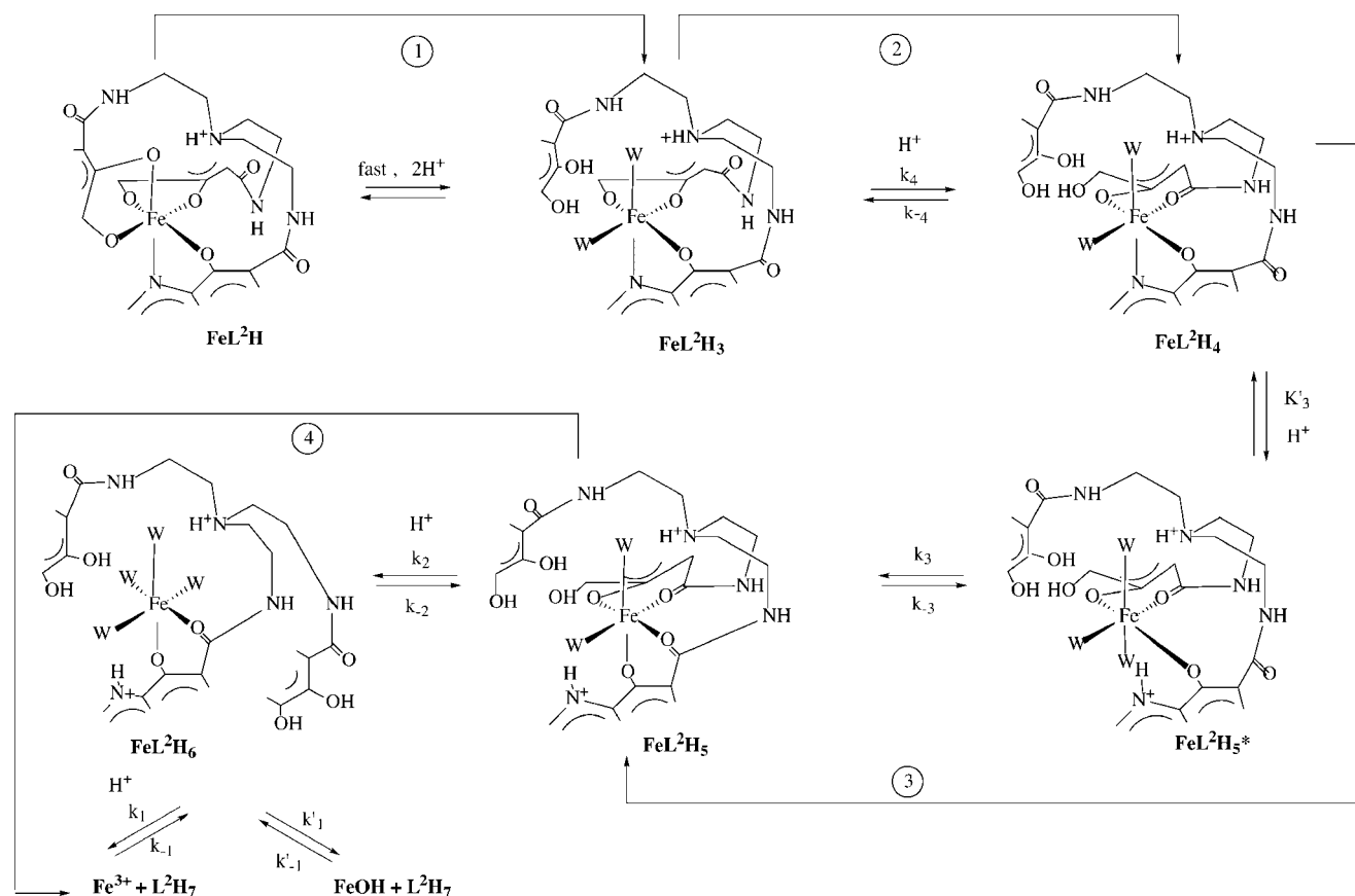
Figure 10. Proposed mechanism for the acid hydrolysis of the \text{FeL}^2\text{H} complex
