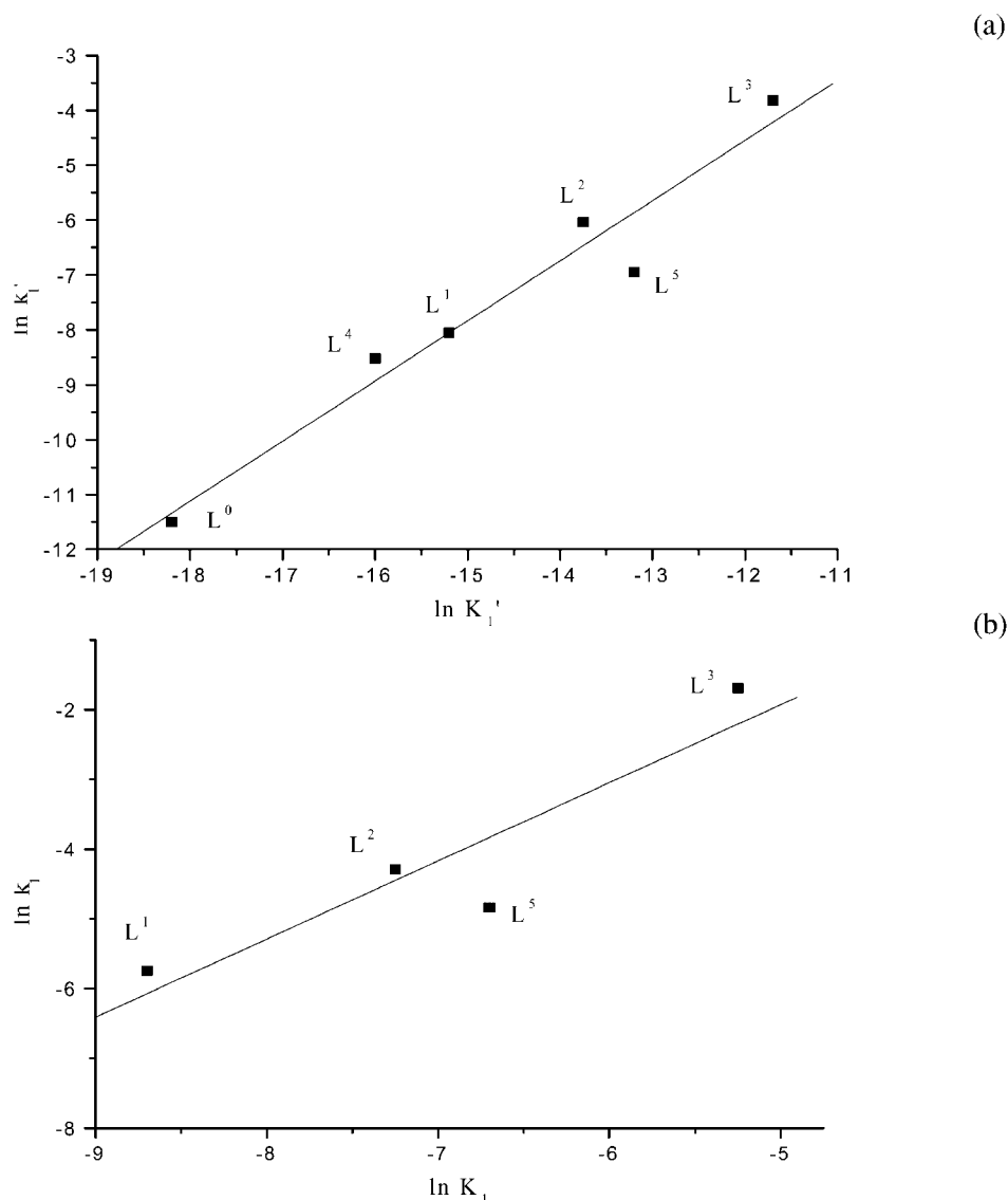
Figure 13. (a) \ln k_1' vs. \ln K_1' for proton-independent dissociation of bidentate Fe– L^n complexes; (b) \ln k_1 vs. \ln K_1 for proton-dependent dissociation of bidentate Fe– L^n complexes; data were measured in aqueous 2.0 M NaClO 4 /HClO 4 at 25 °C
