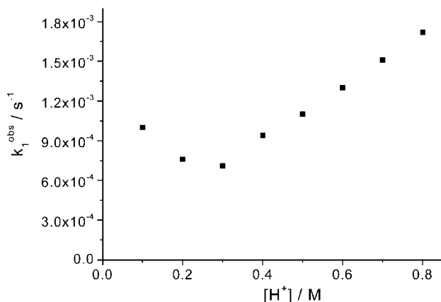
Figure 5. k_1^{\text{obs}} [ \text{s}^{-1} ] as a function of [\text{H}^+] [M] in the acid hydrolysis kinetics of \text{FeL}^1 ; [\text{FeL}^1] = 0.07 \text{ mM} ; solvent: water, I = 2 \text{ M} ( \text{NaClO}_4 , \text{HClO}_4 ), 25^\circ\text{C}
