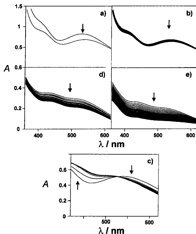
Figure 4. UV/Vis spectra recorded as a function of the time for the acid hydrolysis kinetics of the \text{Fe}^{\text{III}}\text{L}^2 complex: (a) stage 1, 0–3 ms (b) stage 2, 0–1 s (c) stage 3, 0–500 ms (d) stage 4, step 1 0–0.5 s, (e) stage 4, step 2, 0.5–100 s; experimental conditions: see Figure 3; the arrow indicates the direction of change as the reaction proceeds
