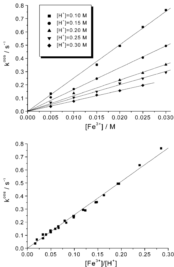
Figure 9. Complex formation kinetics of \text{L}^1 with \text{Fe}^{\text{III}} : (a) k_{\text{obs}} [ \text{s}^{-1} ] as a function of [\text{Fe}^{3+}]_{\text{tot}} [M] at various [\text{H}^+] [M]; [\text{L}^1] = 0.1 \text{ mM} ; (b) k_{\text{obs}} [ \text{s}^{-1} ] as a function of [\text{Fe}^{3+}]/[\text{H}^+] according to Equation (25); solvent: water, I = 2 \text{ M} ( \text{NaClO}_4 , \text{HClO}_4 ), 25^\circ\text{C}
