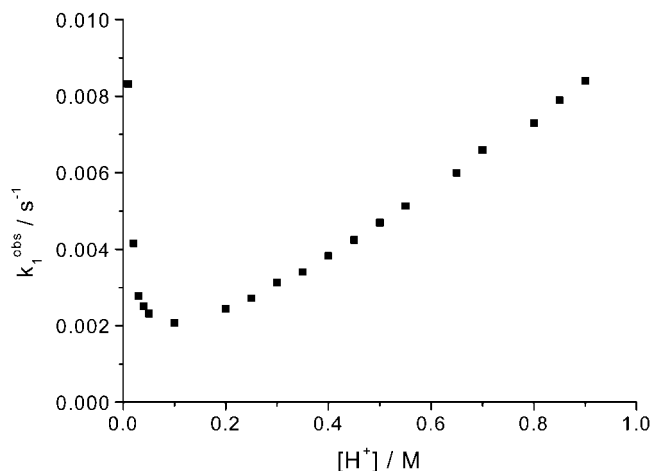
Figure 8. k_1^{\text{obs}} [s -1 ] as a function of [H + ] [M] in the acid hydrolysis kinetics of FeL 5 ; [FeL 5 ] = 0.2 mM; solvent: water, I = 2 M (NaClO 4 , HClO 4 ), 25 °C
