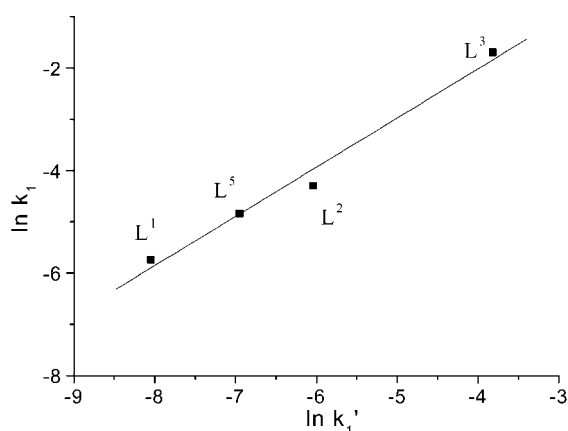
Figure 11. \ln k_1 vs. \ln k_{-1}' for the final step dissociation of \text{FeL}^n complexes; data were measured in aqueous 2.0 M \text{NaClO}_4/\text{HClO}_4 at 25 °C
