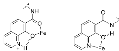
Figure 2. Salicylate (a) and 8-hydroxyquinolate (b) mode of coordination of L with Fe III
